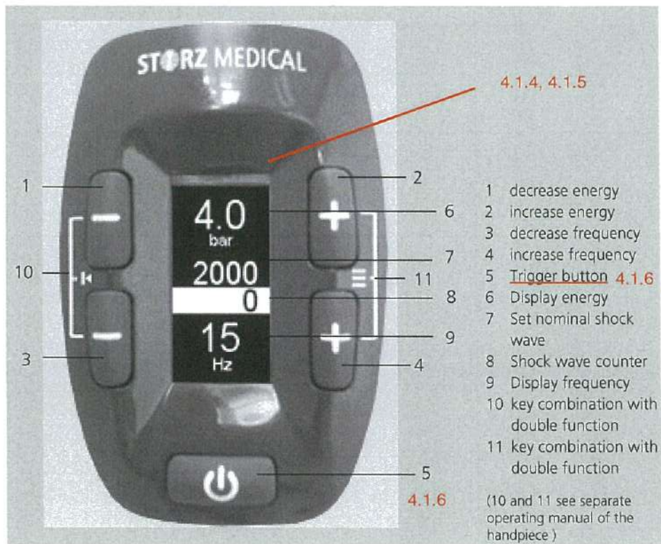
Fig. 4-2 Display and setting buttons of the R-SW handpiece 4.1.4, 4.1.5
